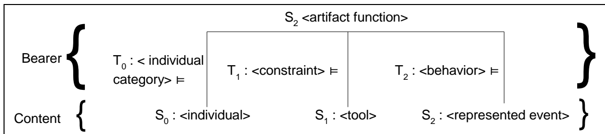
Figure 4. Structure of the metadata modules.
