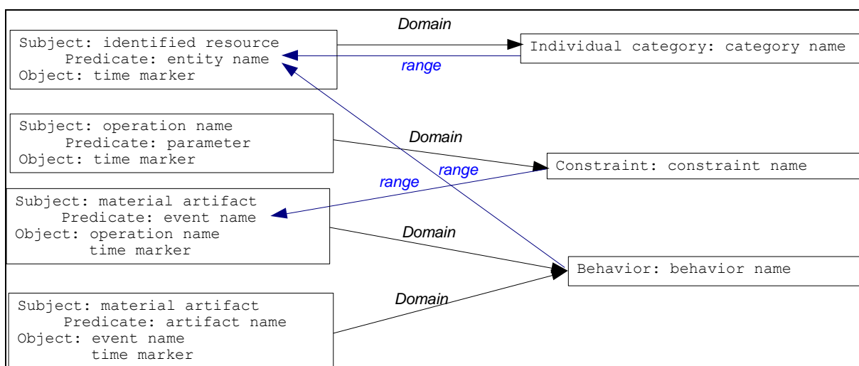
Figure 6. Schematic representation of the inferences between situations and types.
